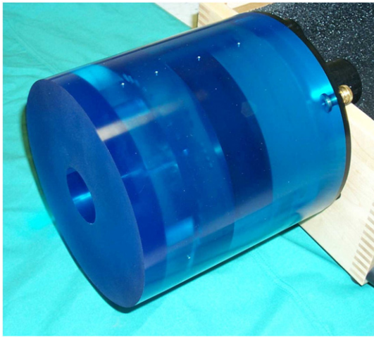
Fig. 2. The CT phantom. This phantom has several regions to test image quality such as low contrast detectability and spatial resolution.
